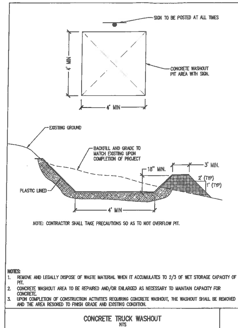
EC02 2 CONCRETE WASHOUT NOT TO SCALE
